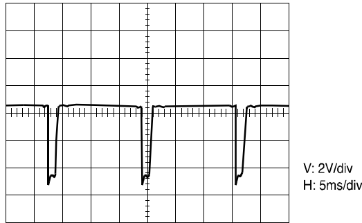
(10) I701 PIN 17
