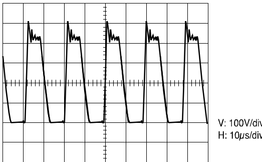
(12) I801 PIN 2
