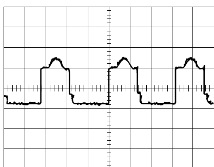
(19) Q403 COLLECTOR
