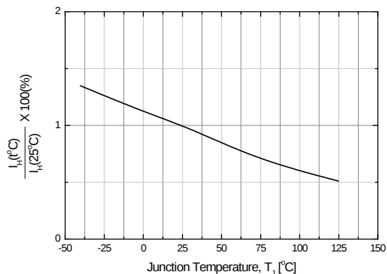
Fig 7. Holding current vs. Junction temperature
