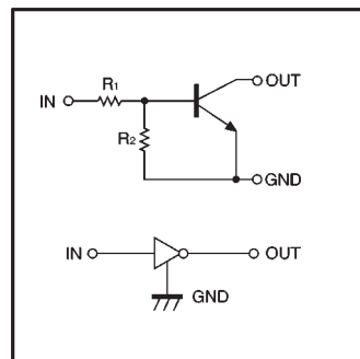
●Equivalent circuit
