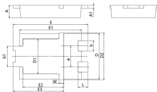
Dimensions-TO-277B
