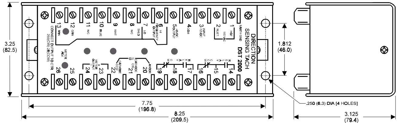
Figure 1-1 Outline Drawing
