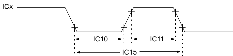
FIGURE 23-9: INPUT CAPTURE (CAPx) TIMING CHARACTERISTICS
