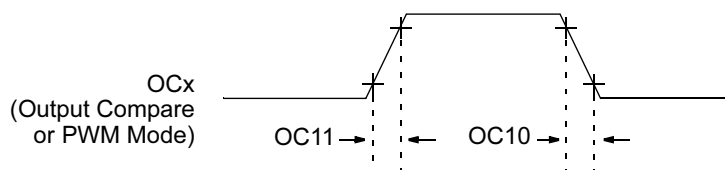
FIGURE 23-10: OUTPUT COMPARE MODULE (OCx) TIMING CHARACTERISTICS
