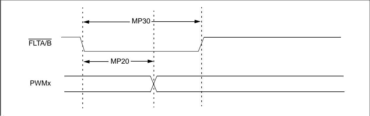
FIGURE 23-13: MOTOR CONTROL PWM MODULE TIMING CHARACTERISTICS
