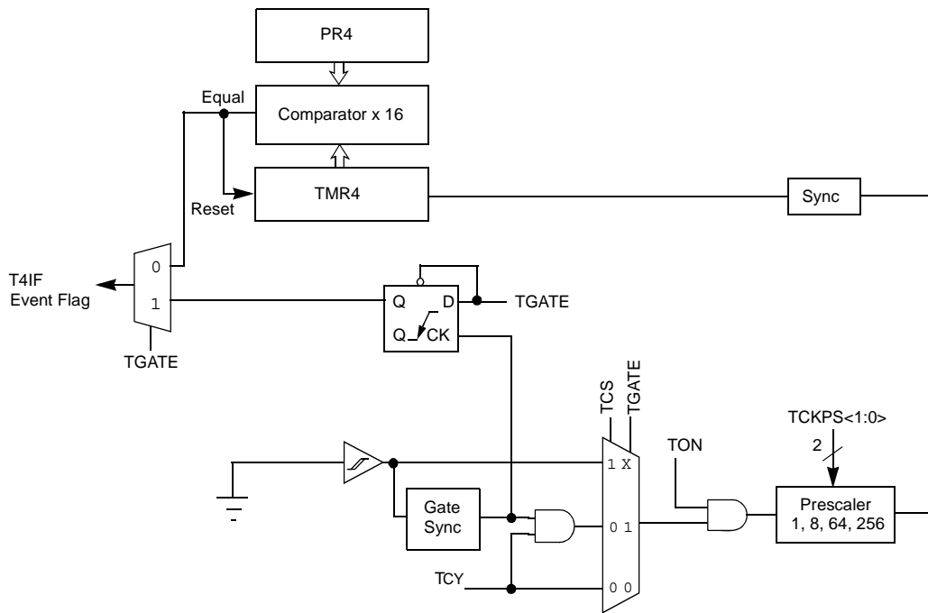
FIGURE 11-2: 16-BIT TIMER4 BLOCK DIAGRAM (TYPE B TIMER)
