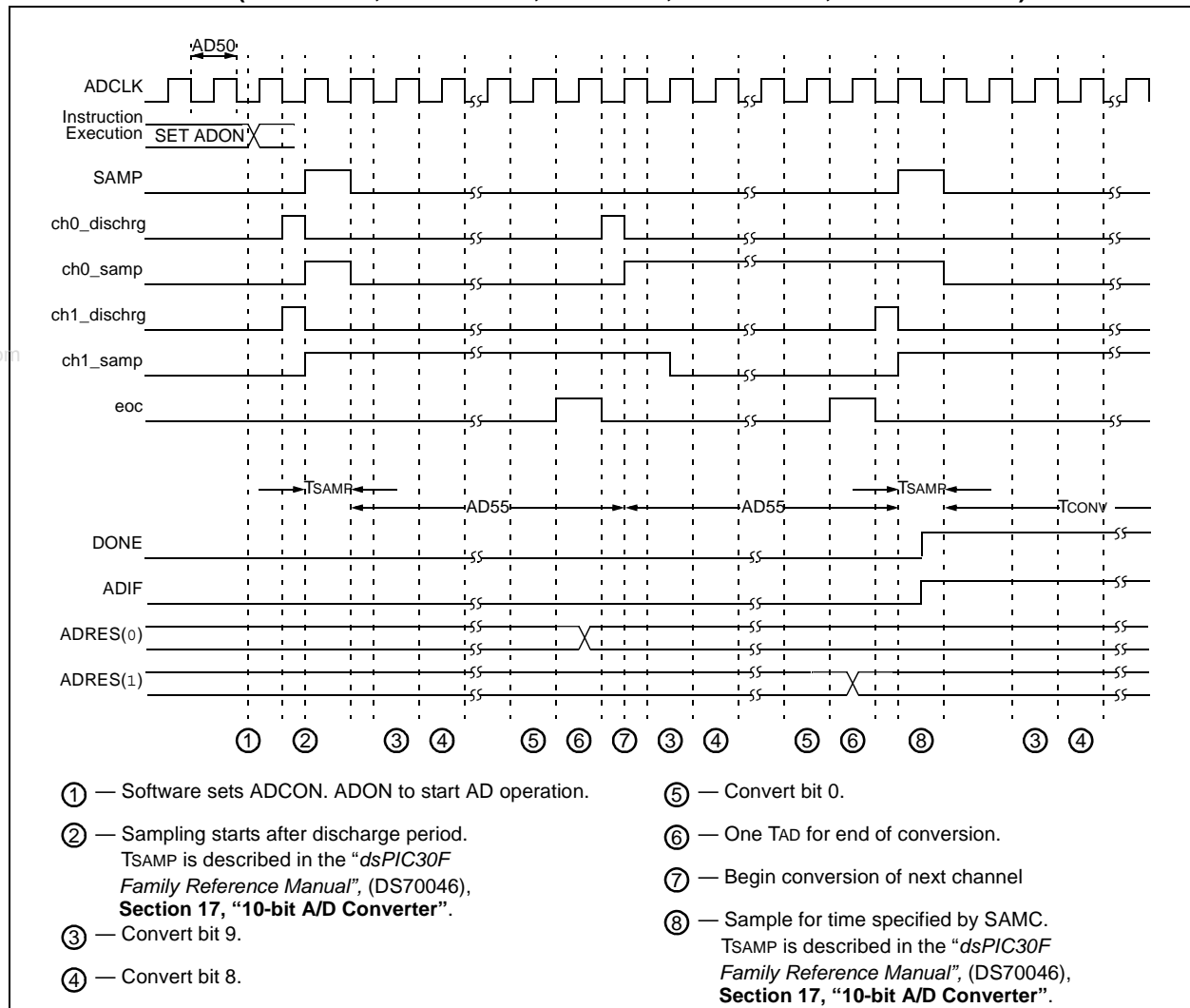
FIGURE 23-25: 10-BIT HIGH-SPEED ADC TIMING CHARACTERISTICS (CHPS = 01, SIMSAM = 0, ASAM = 1, SSR = 111, SAMC = 00001)
