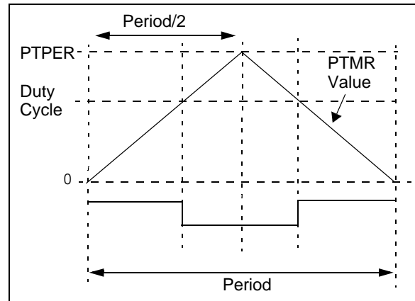
FIGURE 14-3: CENTER-ALIGNED PWM
