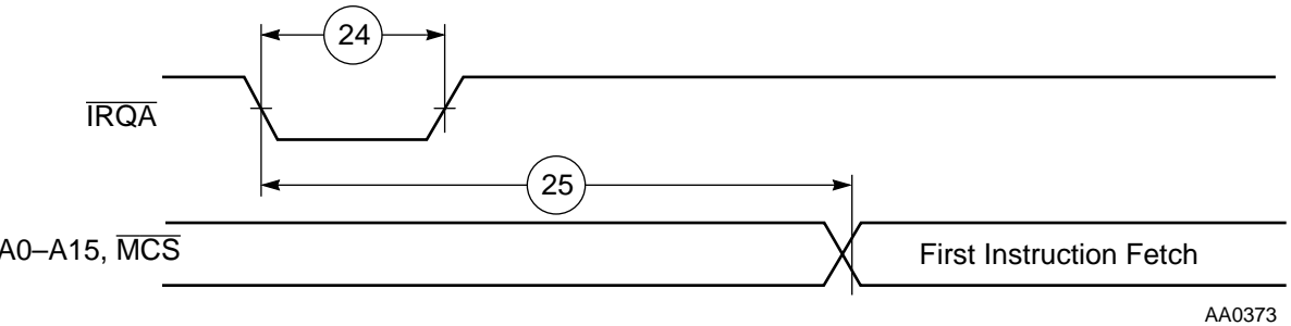
Figure 2-9 Recovery from Stop Using \overline{\text{IRQA}}
