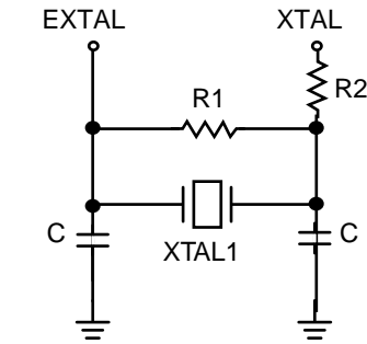
Fundamental Frequency Fork Crystal Oscillator
