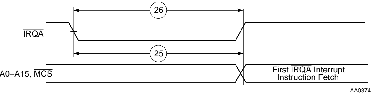
Figure 2-10 Recovery from Stop Using \overline{\text{IRQA}} Interrupt Service
