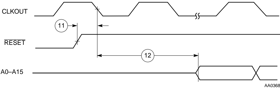
Figure 2-4 Synchronous Reset Timing
