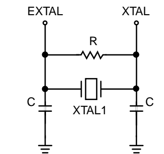
Fundamental Frequency Crystal Oscillator
