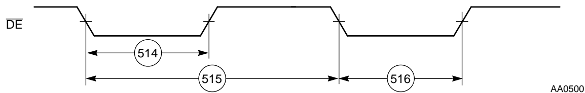
Figure 2-29 OnCE—Debug Request
