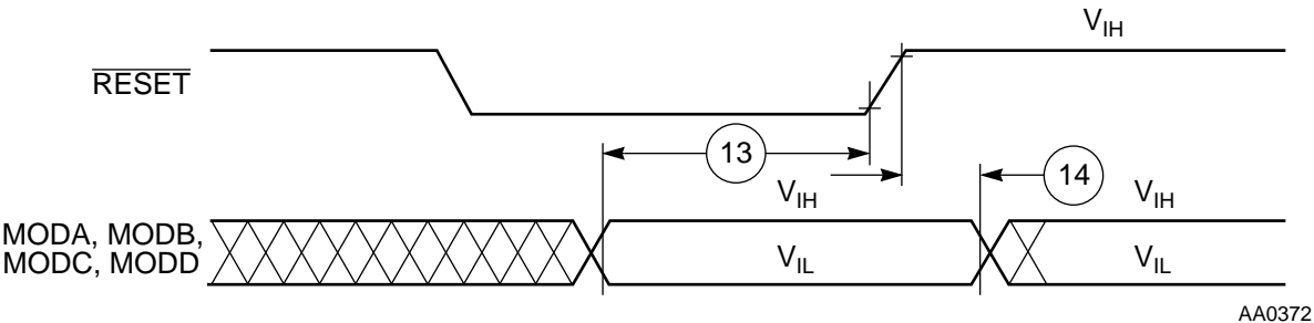
Figure 2-8 Operating Mode Select Timing
