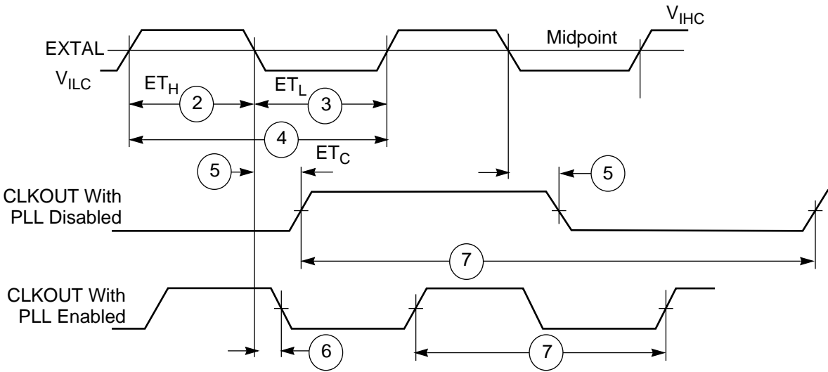
Note: The midpoint is 0.5 (V IHC + V ILC ). AA0367
