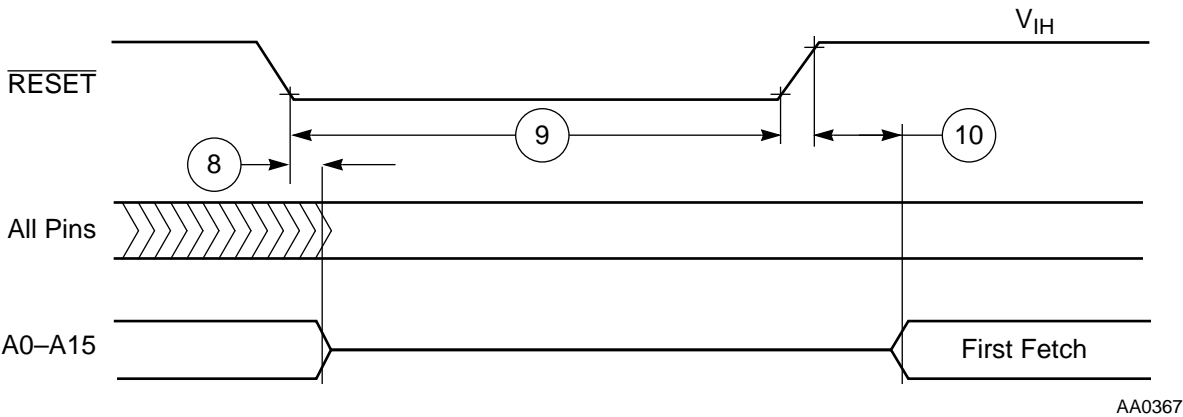
Figure 2-3 Reset Timing
