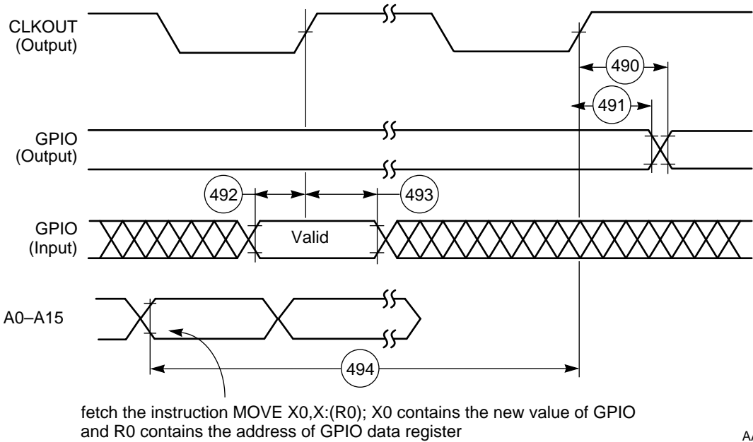
Figure 2-24 GPIO Timing
