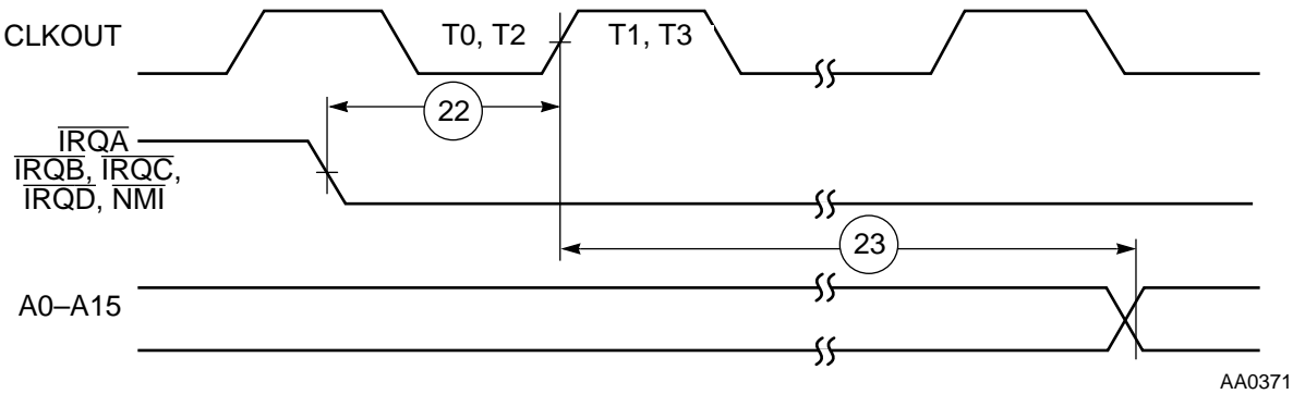
Figure 2-7 Synchronous Interrupt from Wait Timing
