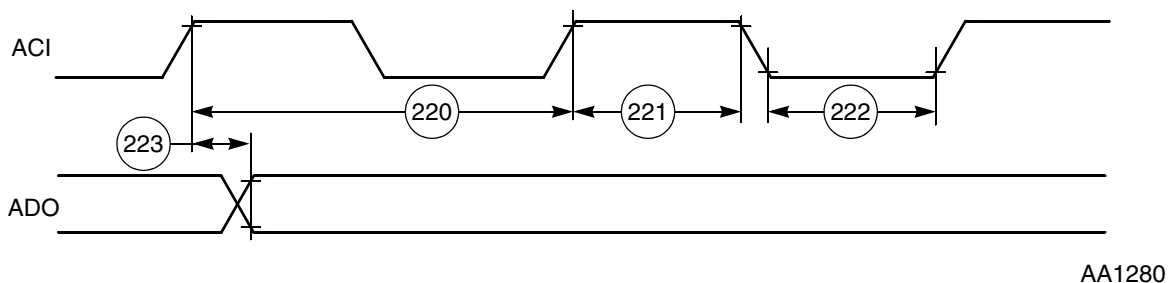
Figure 3-36 Digital Audio Transmitter Timing
