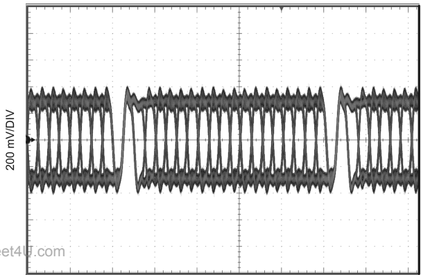
Serial Output Dual Mode, 50 MHz, VSEL = H, No Pre-Emphasis
