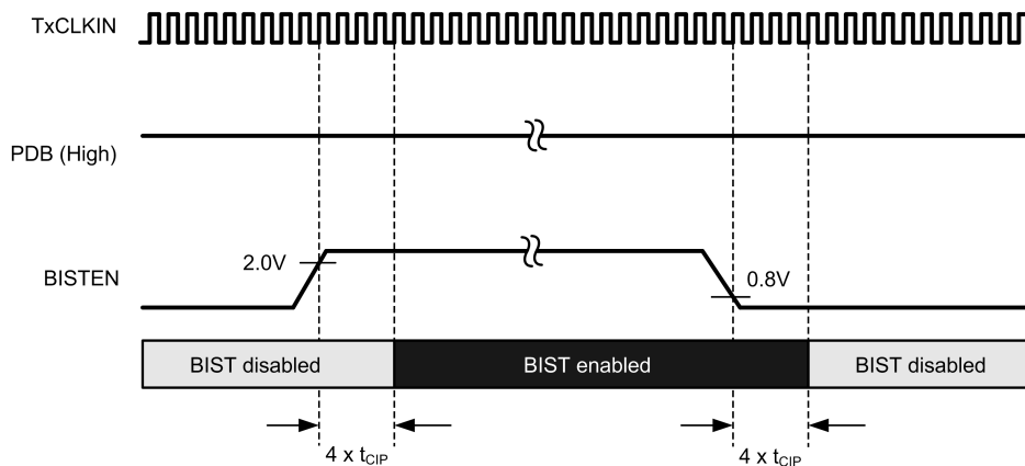
FIGURE 18. BIST Test Enabled/Disabled
