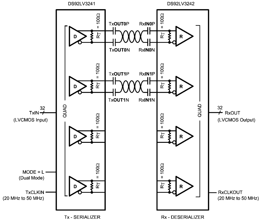
FIGURE 1. Dual Mode
