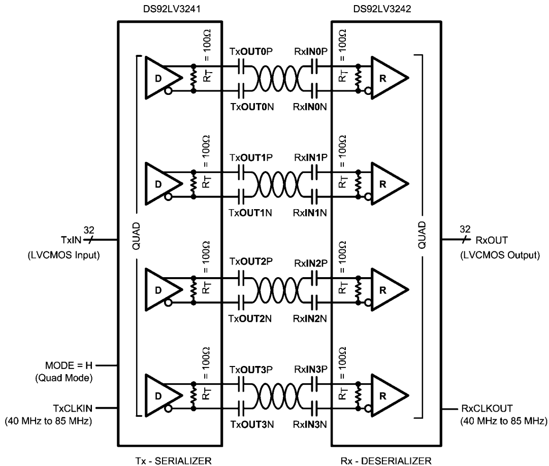
FIGURE 2. Quad Mode
