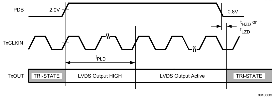
FIGURE 9. Serializer PLL Lock Time
