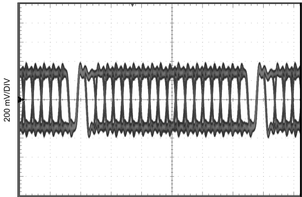
Serial Output Quad Mode, 85 MHz, VSEL = H, No Pre-Emphasis
