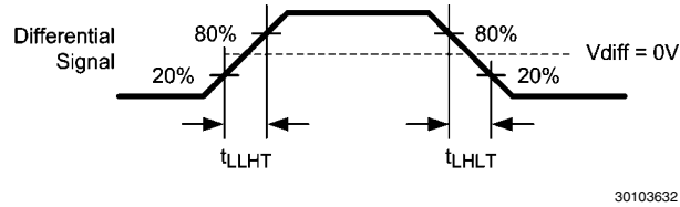
FIGURE 5. Serializer LVDS Transition Times
