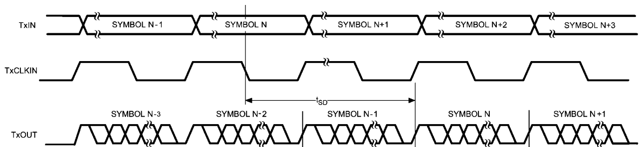
FIGURE 8. Serializer Propagation Delay
