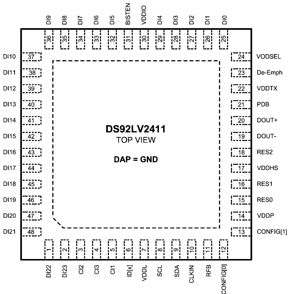
Serializer - DS92LV2411 — Top View
