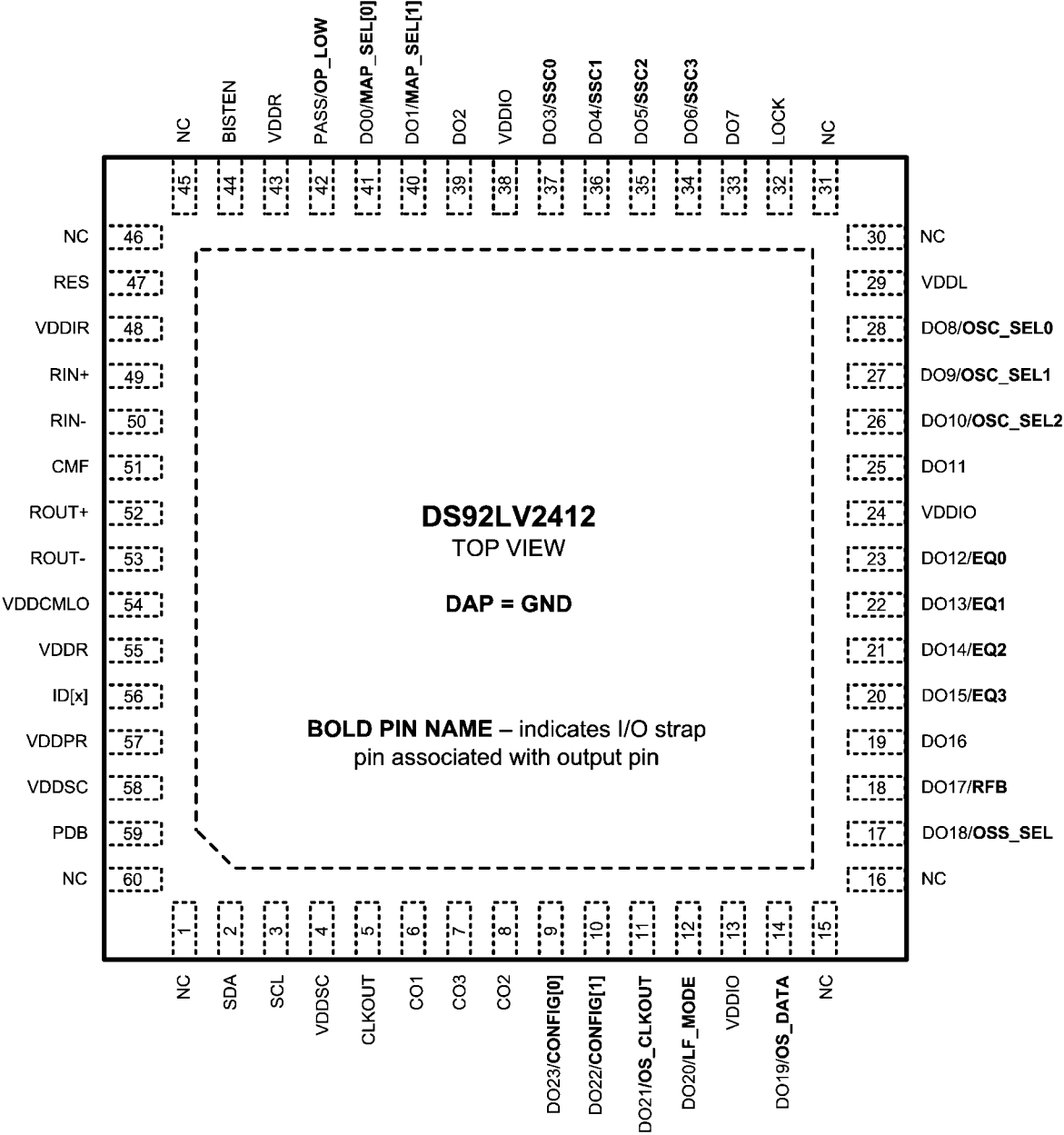
Deserializer - DS92LV2412 — Top View
