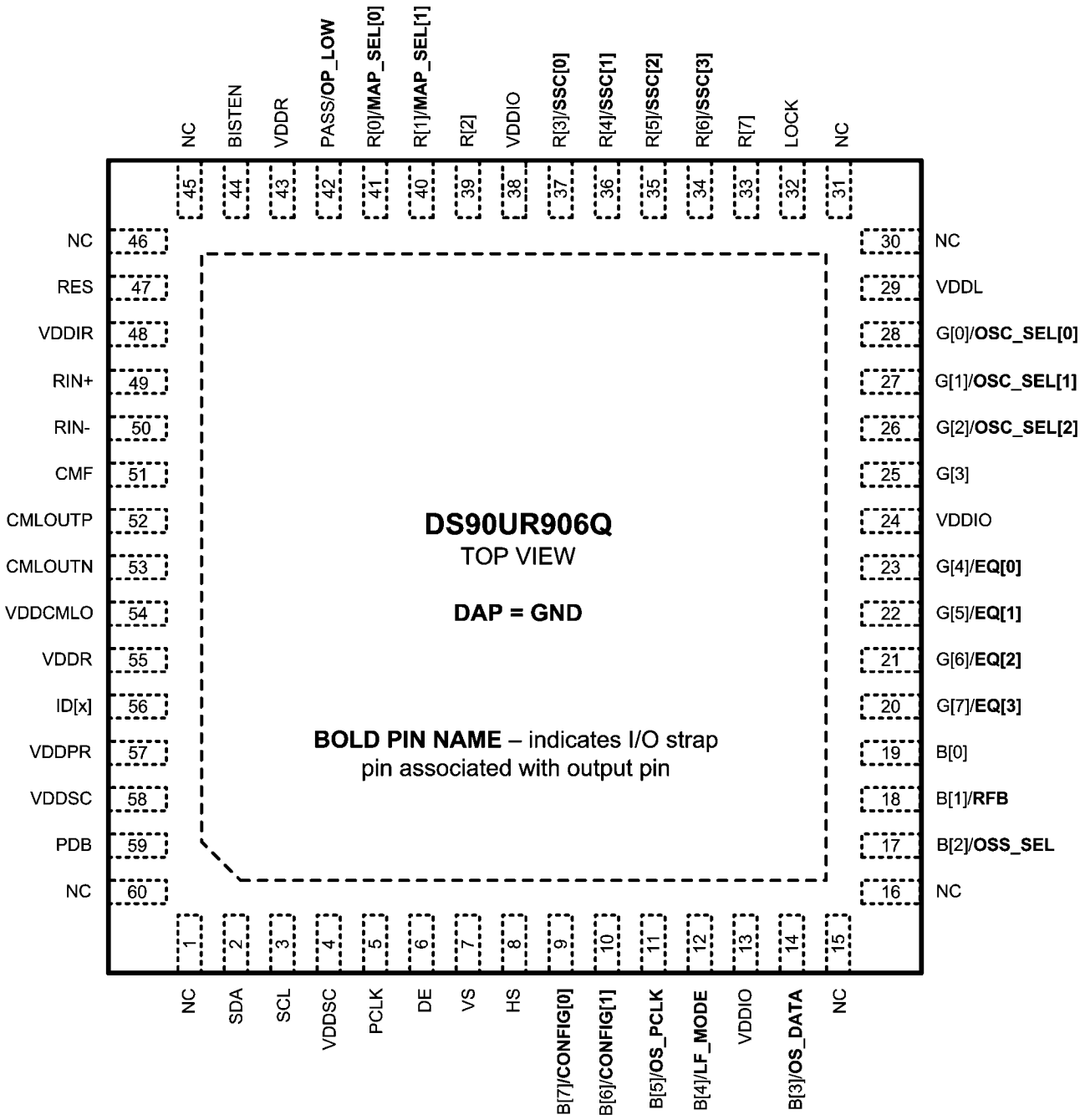
Deserializer - DS90UR906Q — Top View
