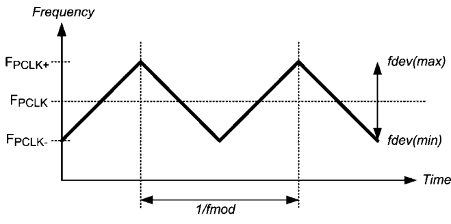
FIGURE 22. SSCG Waveform
