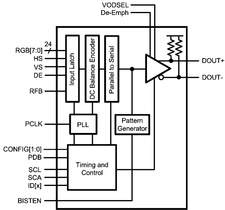
DS90UR905Q – SERIALIZER
