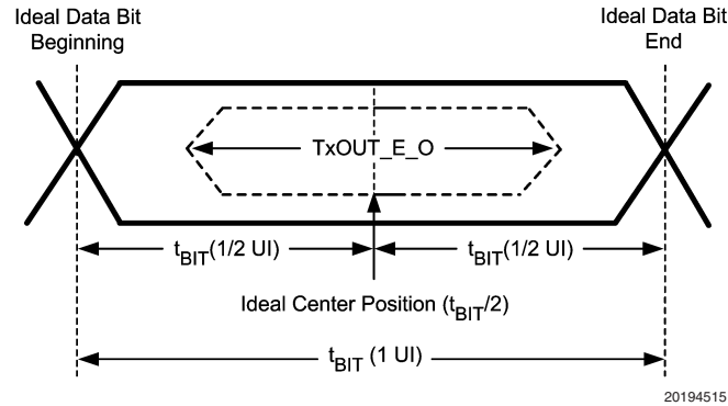
FIGURE 15. Transmitter Output Eye Opening ( TxOUT\_E\_O )
