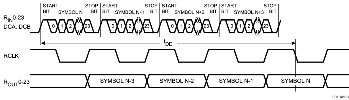
FIGURE 10. Deserializer Delay
