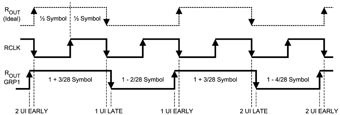
FIGURE 11. Deserializer Setup and Hold Times and PTO, PTOSEL = H
