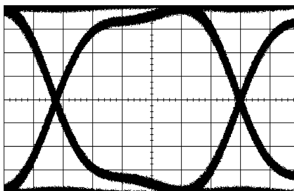
Diff. Output Eye-Pattern in 1:2 split mode @ 800 Mbps Conditions: 3.3 V, PRBS = 2^{23}-1 data pattern, V_{ID} = 300 mV, V_{CM} = +1.2 V, 200 ps/div, 100 mV/div
