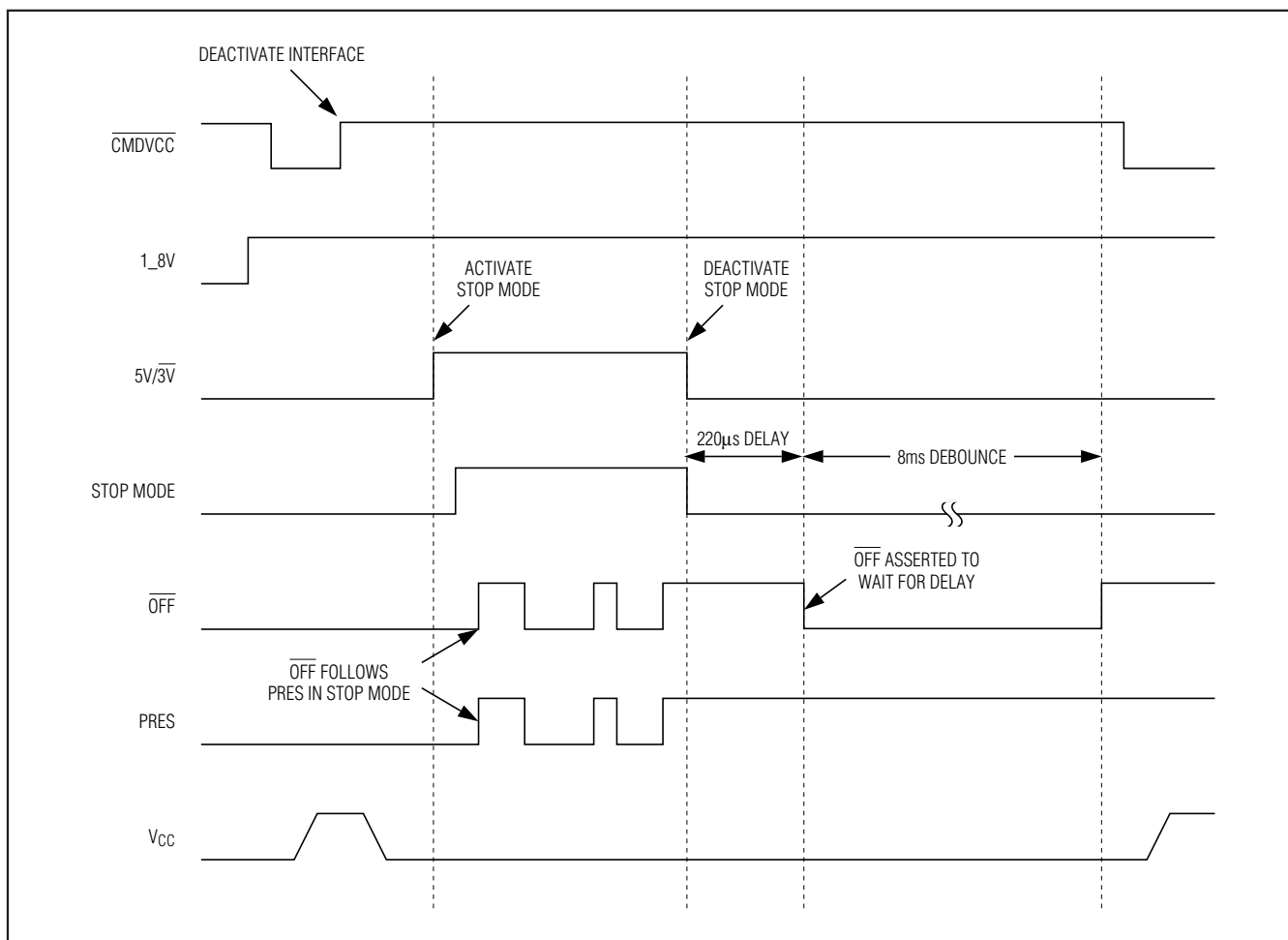
Figure 8. Stop-Mode Sequence
