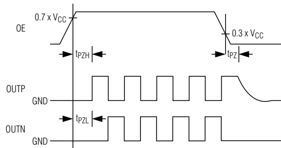
Figure 3. HCSL Output Timing Diagram When OE is Enabled and Disabled
