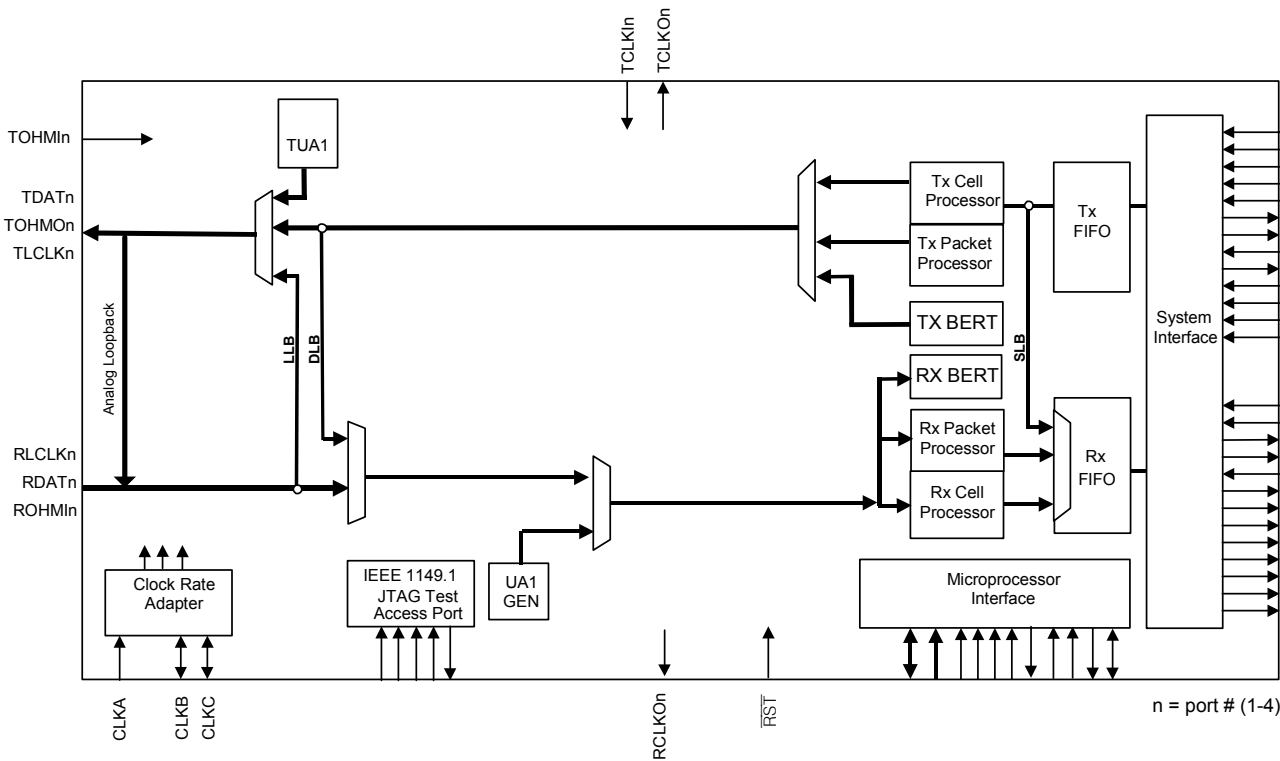
Figure 6-9. Clear-Channel ATM/Packet—OHM Mode
