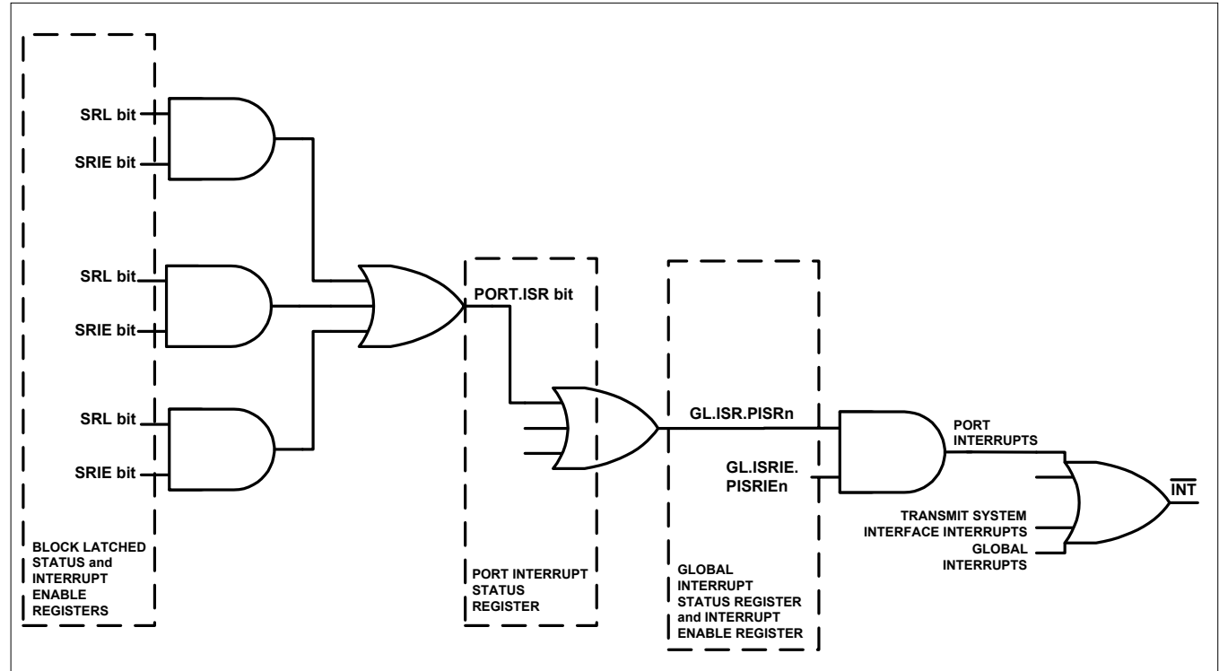
Figure 10-1. Interrupt Structure
