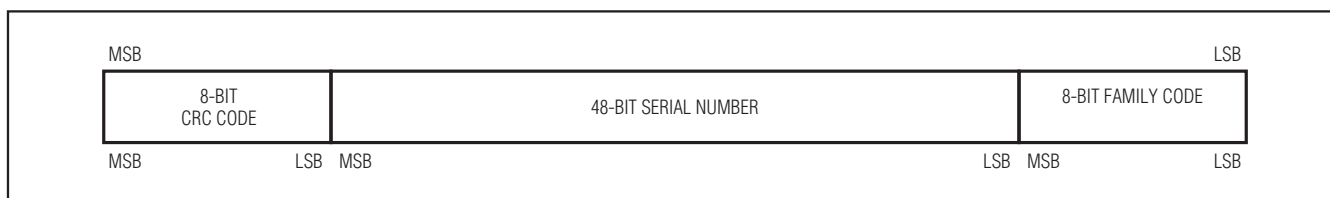
Figure 3. 64-Bit ROM
