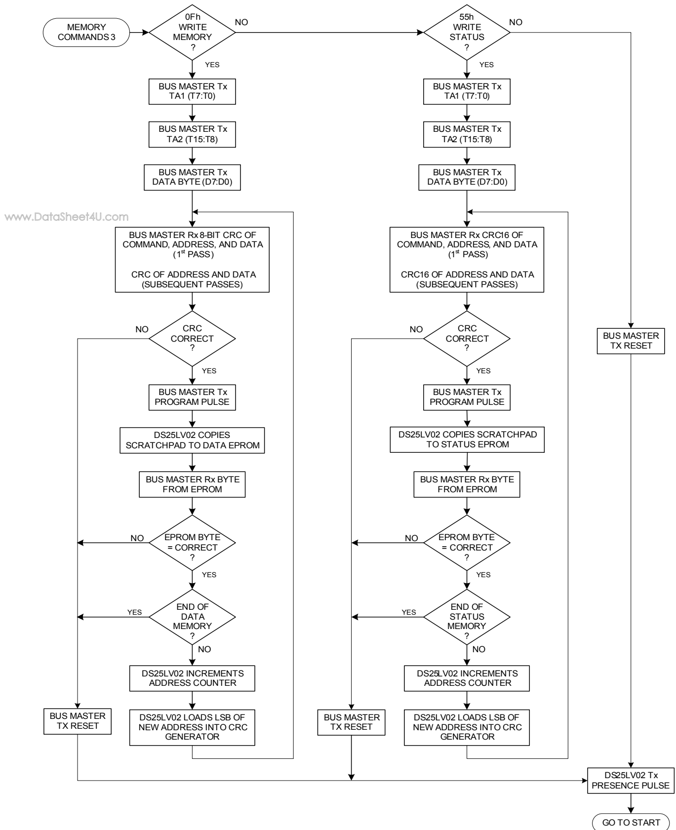
Figure 8. Operational Flow Chart (Continued)
