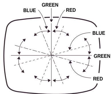
Line movement when adjusting top of yoke in and out.
