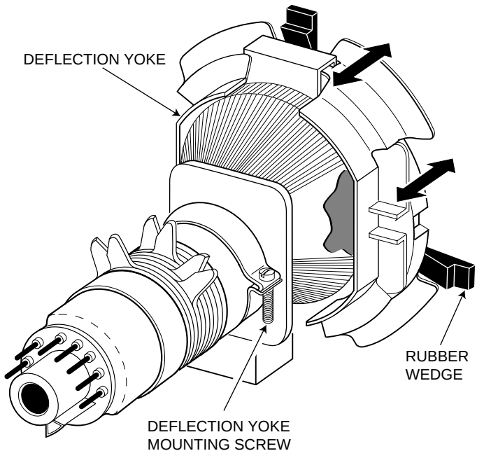
Figure 1. Deflection Yoke Movement
