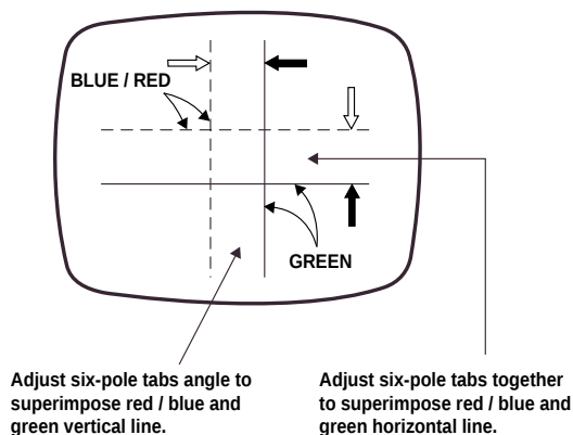
Figure 5. Blue/Red and Green Line Movement
