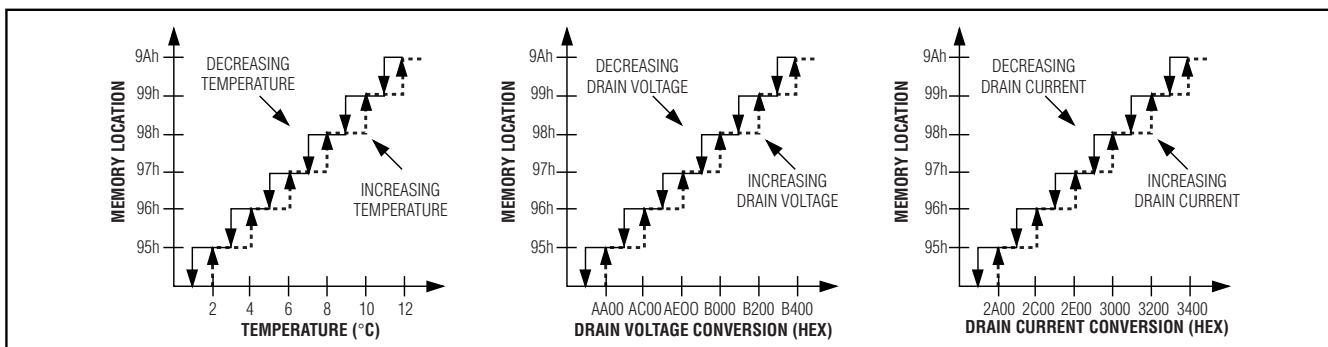
Figure 1. LUT Hysteresis
