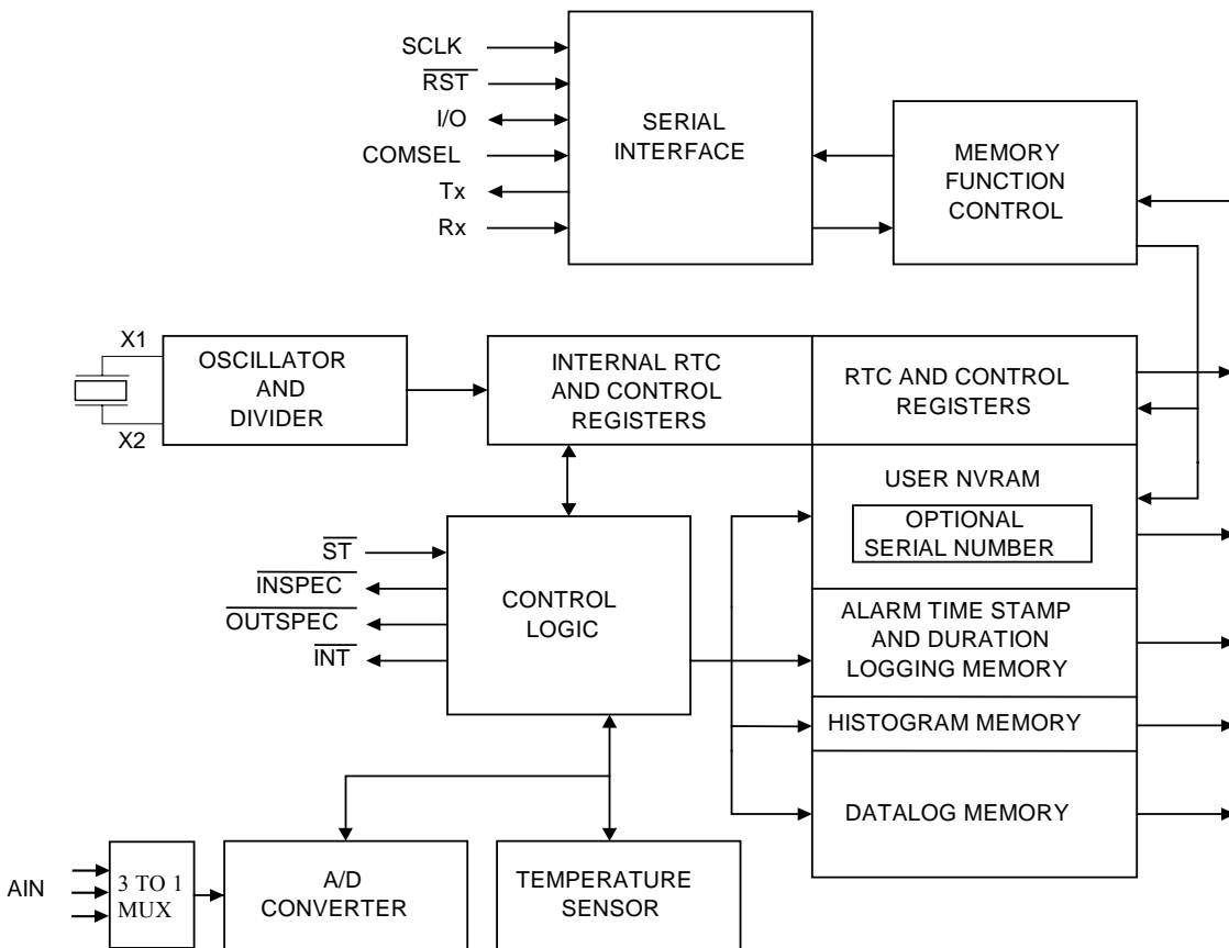
DS1616 Block Diagram Figure 1
