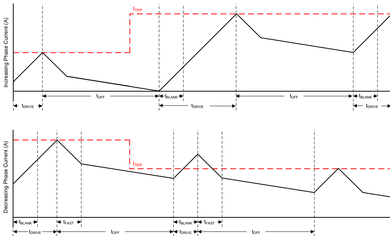
Figure 19. Mixed-Mixed Decay Mode
