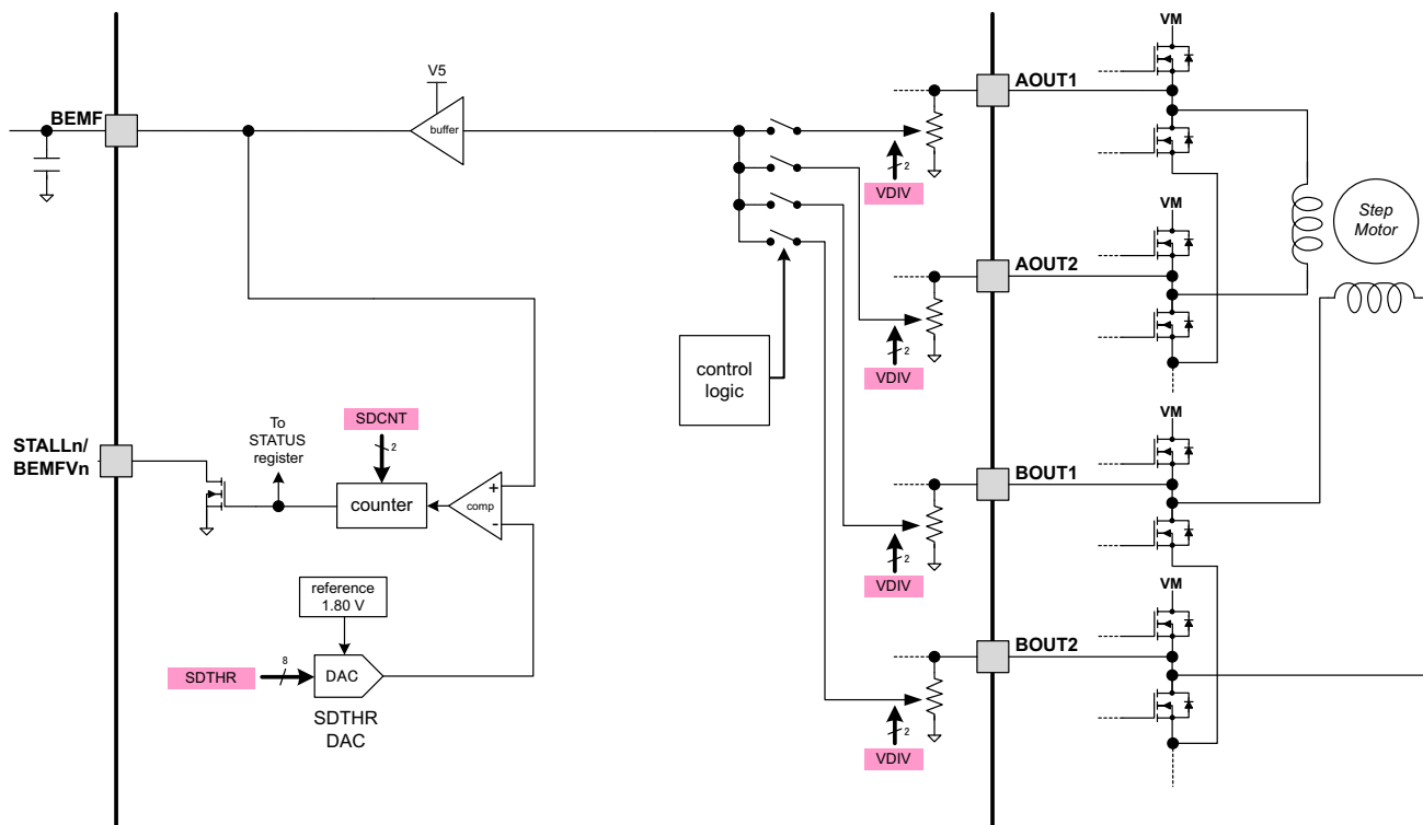
Figure 15. Stall Detection
