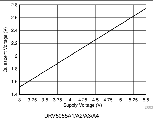
Figure 6-3. Quiescent Voltage vs. Supply Voltage
