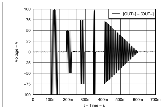
Figure 50. Example Waveform – Pinball Effect
