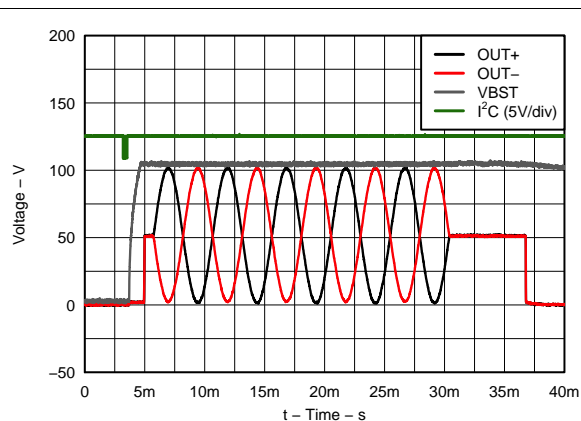
Figure 51. Typical Waveform
