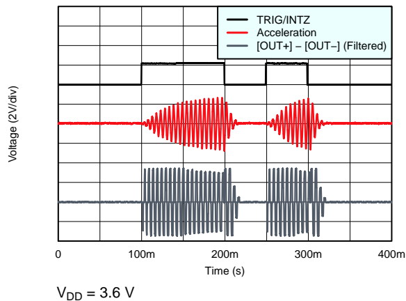
Figure 13. LRA SimpleDrive with Closed-Loop
