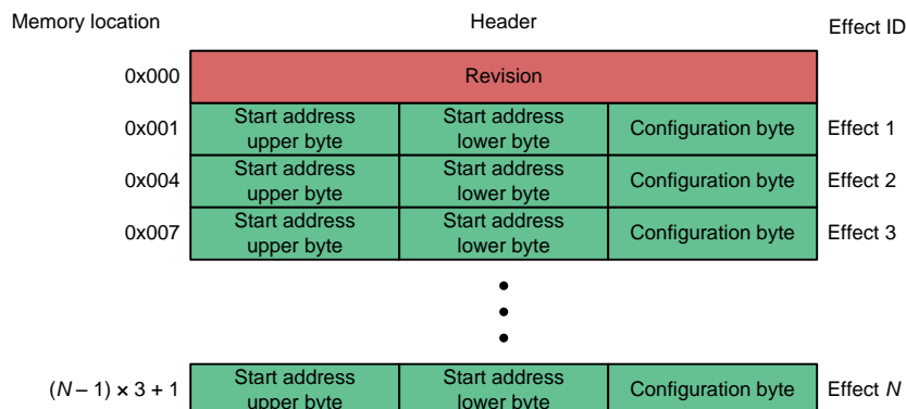
Figure 30. Header Structure
