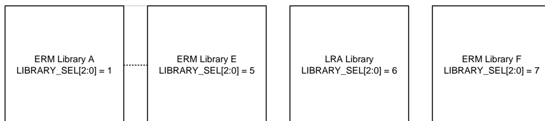
Figure 12. Library Selection
