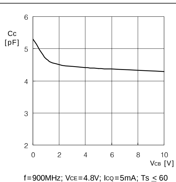
Fig 2. Collector-base capacitance v.s Collector-base voltage(DC)
