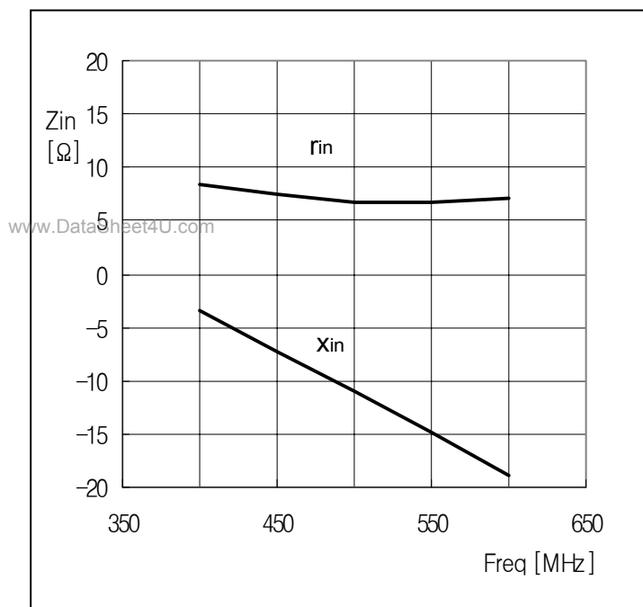
Fig 5. Input Impedance (series components) as a freq, typical values.
