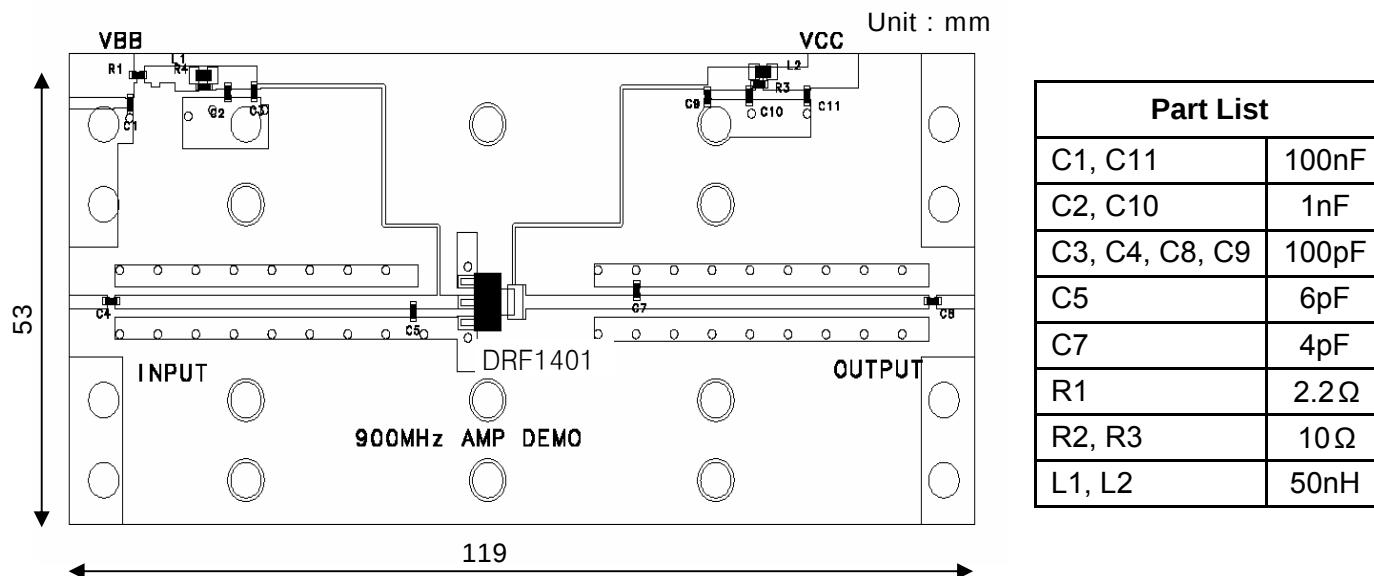
Fig 7. Test Circuit Board Layout @ f = 900\text{MHz}
