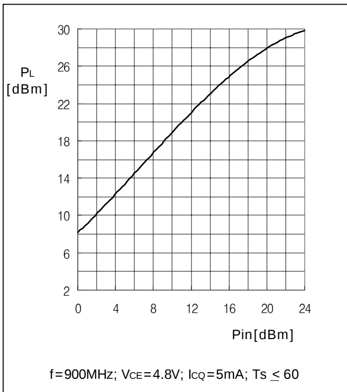
Fig 4. Load power v.s input power (typical value)
