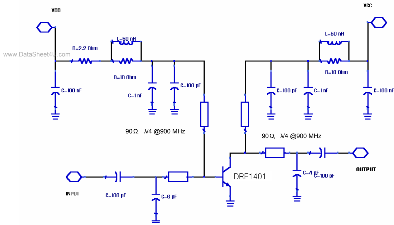
Fig 8. Test Circuit Schematic Diagram @ f = 900\text{MHz}
