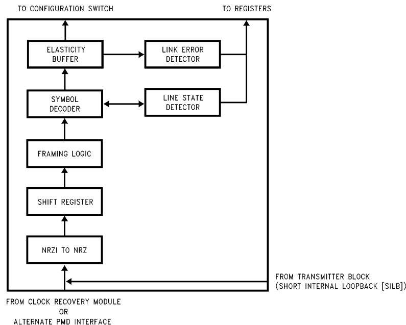
FIGURE 3-2. Receiver Block Diagram
