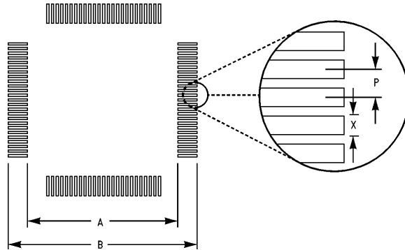
FIGURE 9-1. Layout Land Patterns
