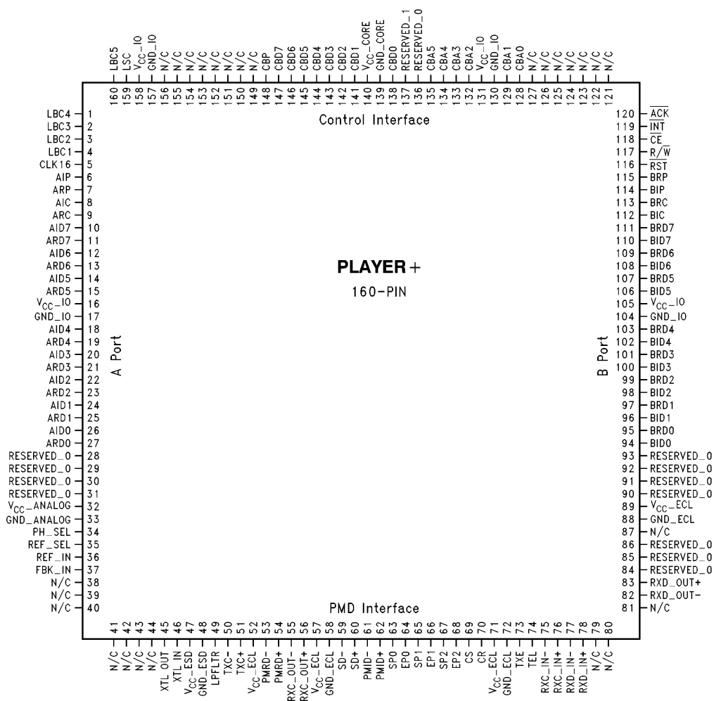
FIGURE 8-3. DP83257VF 160-Pin JEDEC Metric PQFP Pinout
