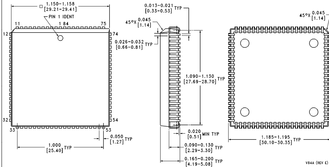
Plastic Leaded Chip Carrier Order Number DP83251V NS Package Number V84A
