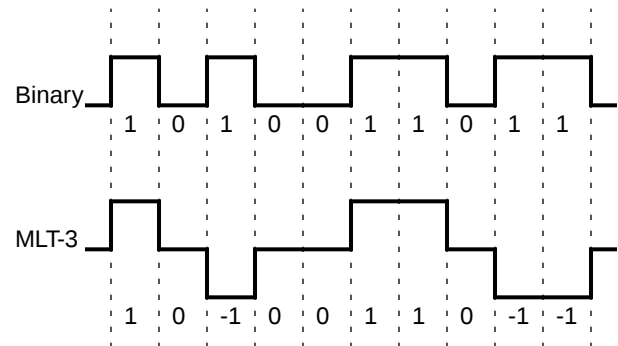
Figure 3-1. Example of Binary vs. MLT-3
