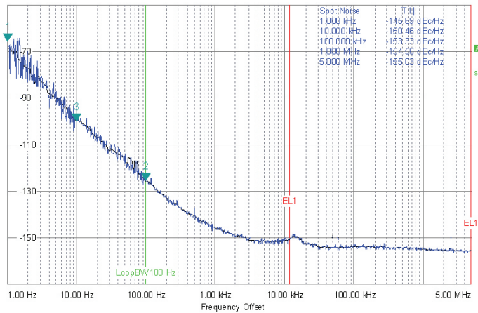
Typical Phase Noise for DOCSC022V-024.576M
