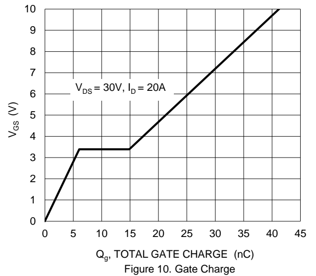
Figure 10. Gate Charge
