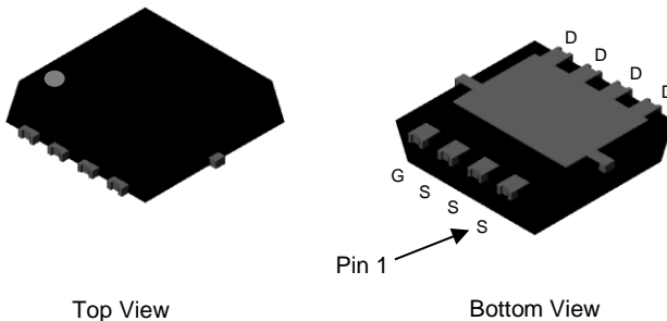
PowerDI3333-8 (SWP) (Type UX)
