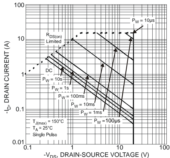
Fig. 8 SOA, Safe Operation Area
