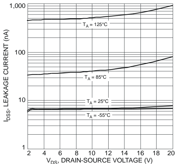
Fig. 14 Typical Leakage Current vs. Drain-Source Voltage
