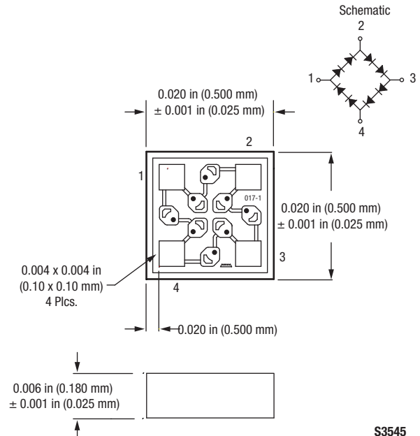
Figure 5. 556-020 Package Dimensions
