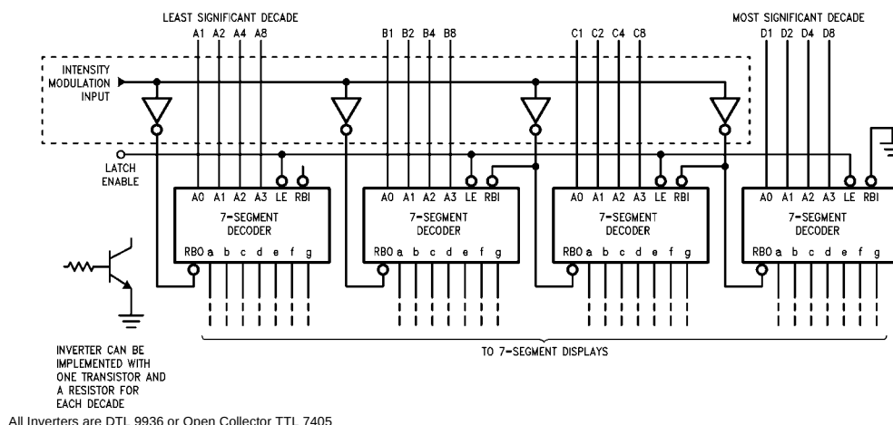
FIGURE 2. Intensity Control by RBO Pulse Duty Cycle
