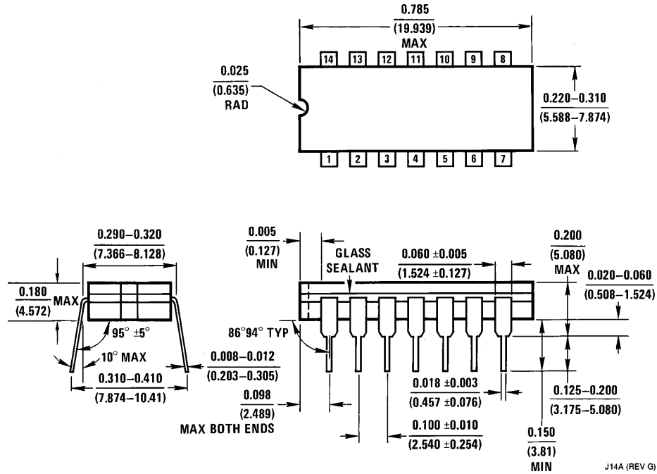
14-Lead Ceramic Dual-In-Line Package (J) Order Number 5474DMQB or DM5474J NS Package Number J14A
