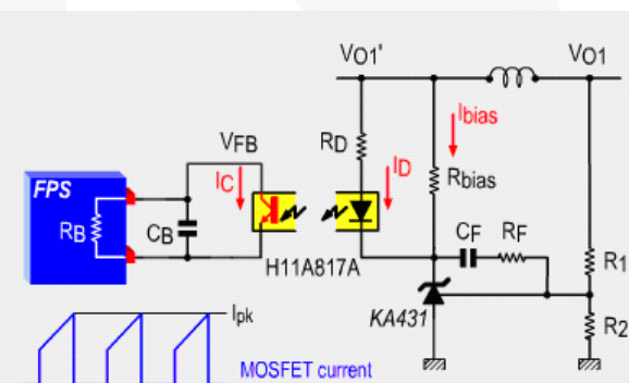
Figure 24. Typical Feedback Network of FPS™
