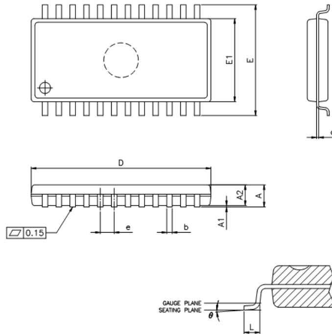
VARIATIONS (ALL DIMENSIONS SHOWN IN MM)
