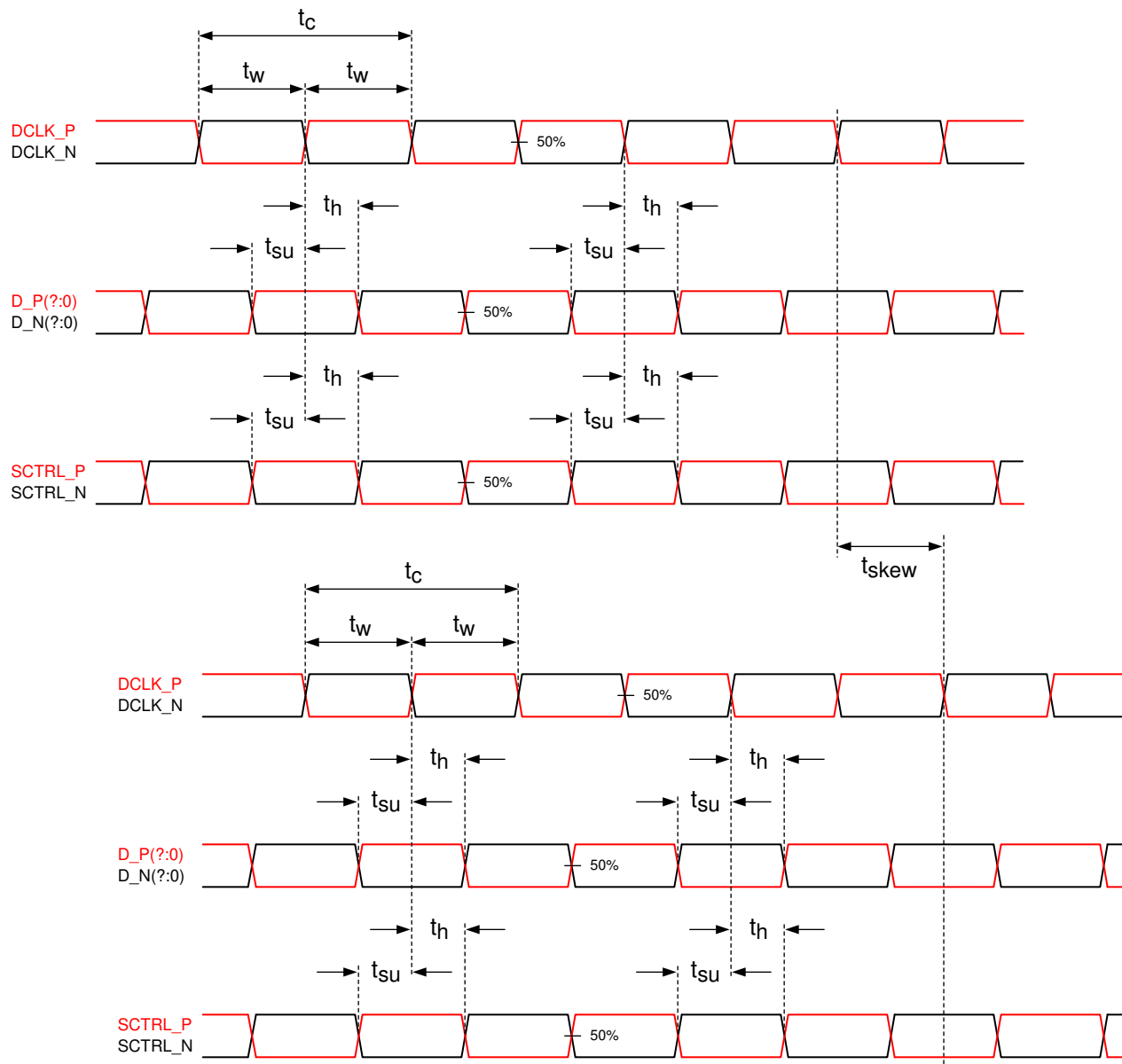
Figure 6-6. Timing Requirements
