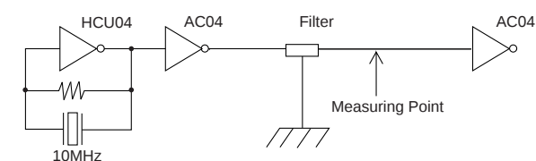
[Testing Circuit]
