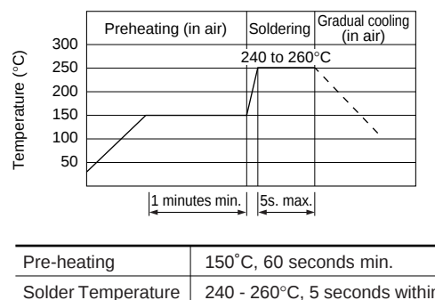
[Flow Soldering]
