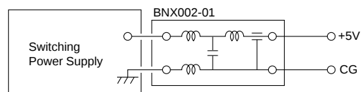
[Testing Circuit]
