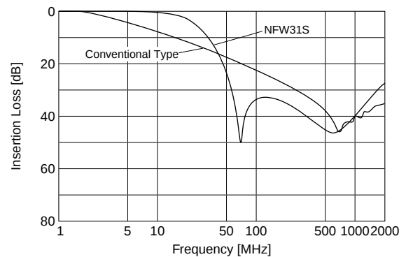
[Comparison of Insertion Loss Characteristics]
