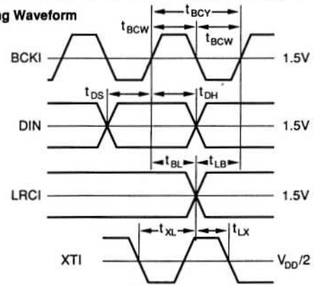
Timing Waveform
