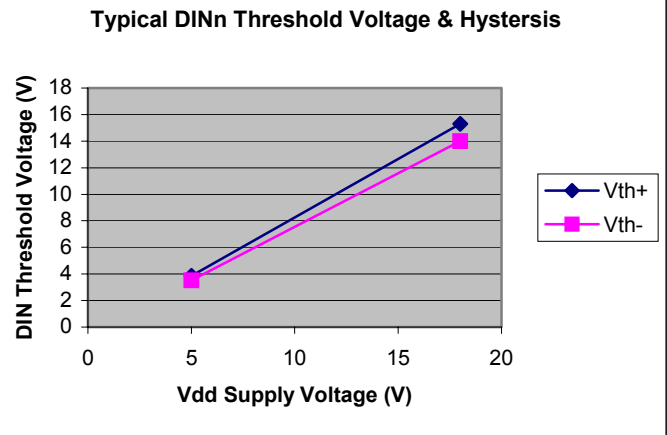
Figure 4 DIN Threshold vs Vdd
