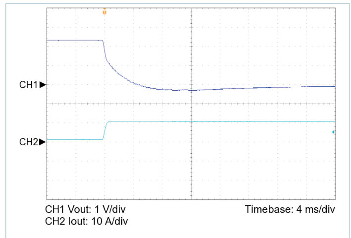
Figure 8 — 10% to 100% load transient response, V_{IN} = 270\text{ V} , nominal trim, C_{OUT\_EXT} = 220\text{ }\mu\text{F}
