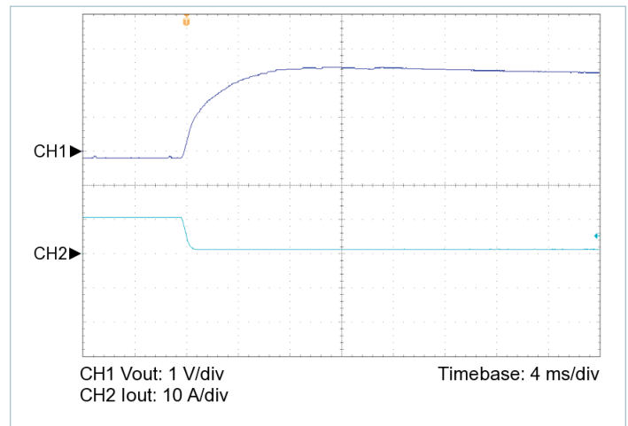
Figure 7 — 100% to 10% load transient response, V_{IN} = 270\text{ V} , nominal trim, C_{OUT\_EXT} = 220\text{ }\mu\text{F}
