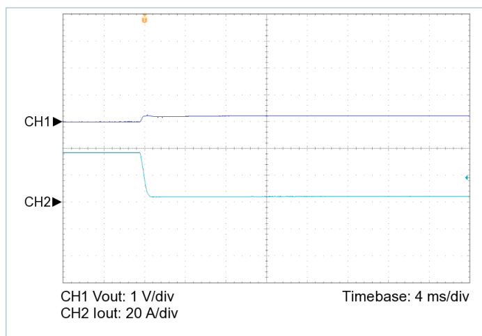
Figure 7 — 100% to 10% load transient response, V_{IN} = 28\text{ V} , nominal trim, C_{OUT\_EXT} = 1000\text{ }\mu\text{F}
