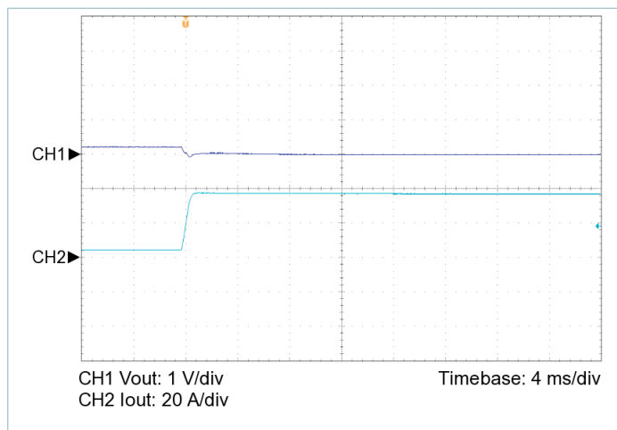
Figure 8 — 10% to 100% load transient response, V_{IN} = 28\text{ V} , nominal trim, C_{OUT\_EXT} = 1000\text{ }\mu\text{F}
