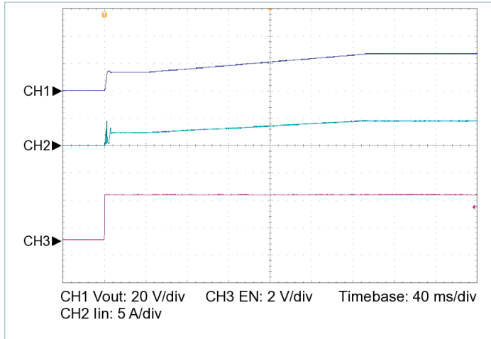
Figure 15 — Startup from EN, V_{IN} = 48\text{ V} , C_{OUT\_EXT} = 2500\text{ }\mu\text{F} , R_{LOAD} = 2.450\text{ }\Omega
