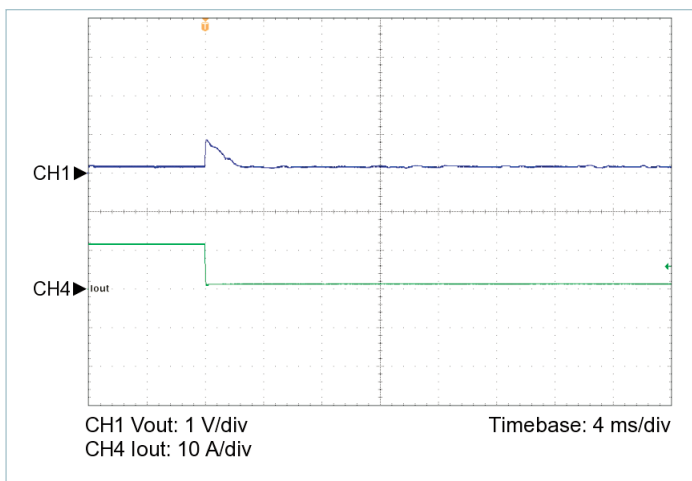
Figure 5 — 100% to 10% load transient response, V_{IN} = 48\text{ V} , nominal trim, C_{OUT\_EXT} = 250\text{ }\mu\text{F}
