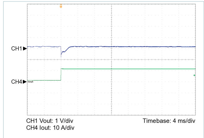
Figure 6 — 10% to 100% load transient response, V_{IN} = 48\text{ V} , nominal trim, C_{OUT\_EXT} = 250\text{ }\mu\text{F}
