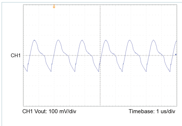
Figure 17 — Output voltage ripple, V_{IN} = 48\text{ V} , V_{OUT} = 28.0\text{ V} , C_{OUT\_EXT} = 250\text{ }\mu\text{F} , R_{LOAD} = 2.450\text{ }\Omega
